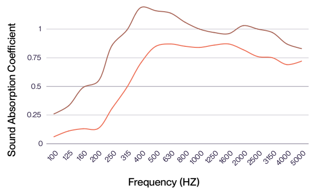
Sound Absorption of PANELS tested to AS ISO 354-2006 Acoustics:
