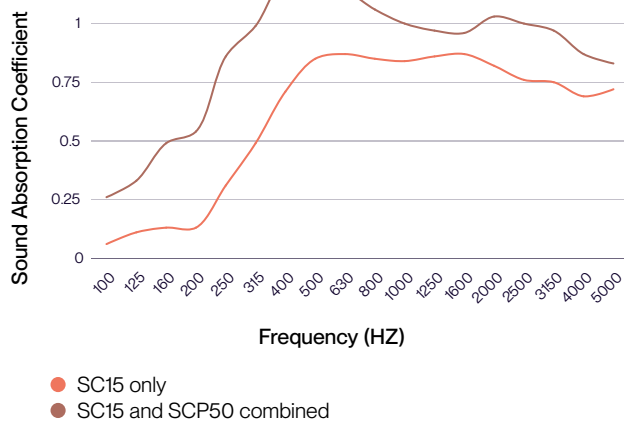
Sound Absorption of PANELS tested to AS ISO 354-2006 Acoustics:
