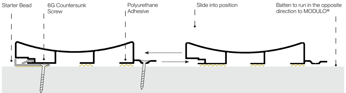
Mating Detail
