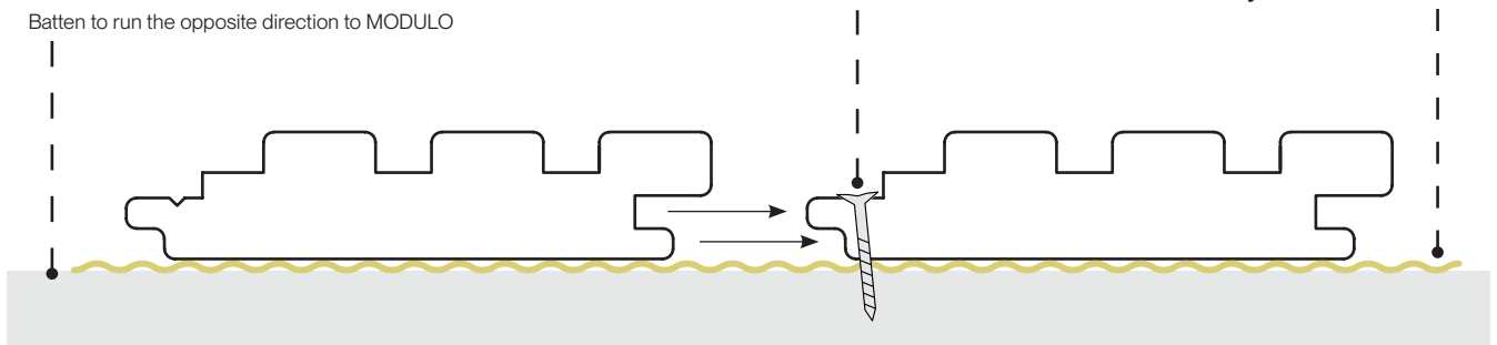
Mating Detail
