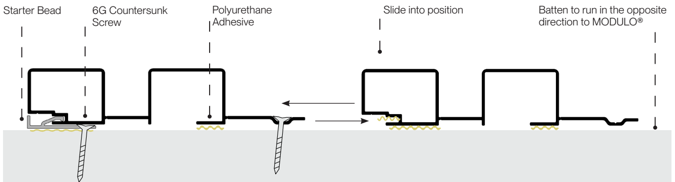
Mating Detail
