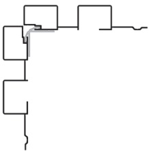
Mating Detail
