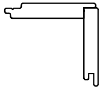
Rebated Corner Detail
