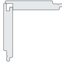
Rebated Corner Detail
