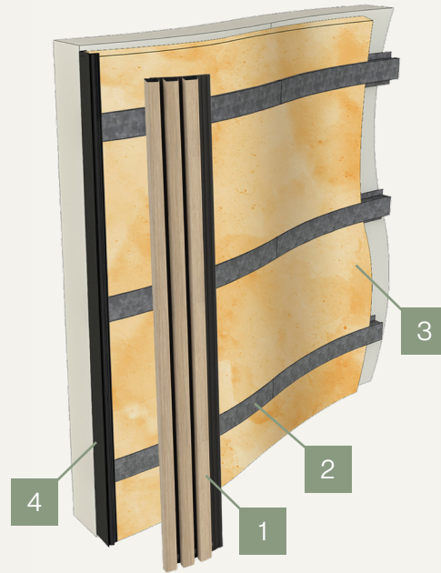
Figure 9. Manipulate to desired radius using discreet fixings
