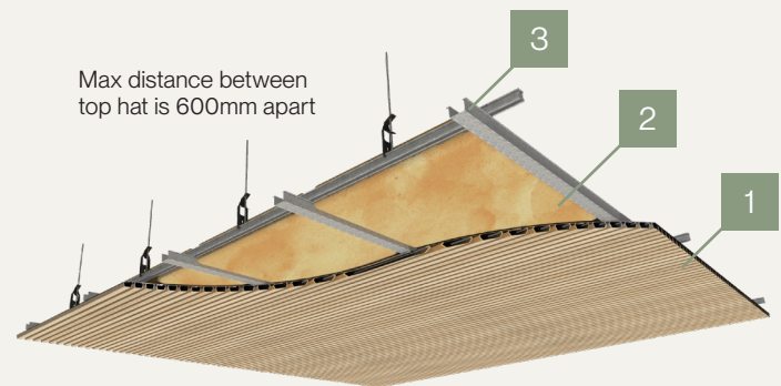
Figure 11. Typical suspended ceiling detail
