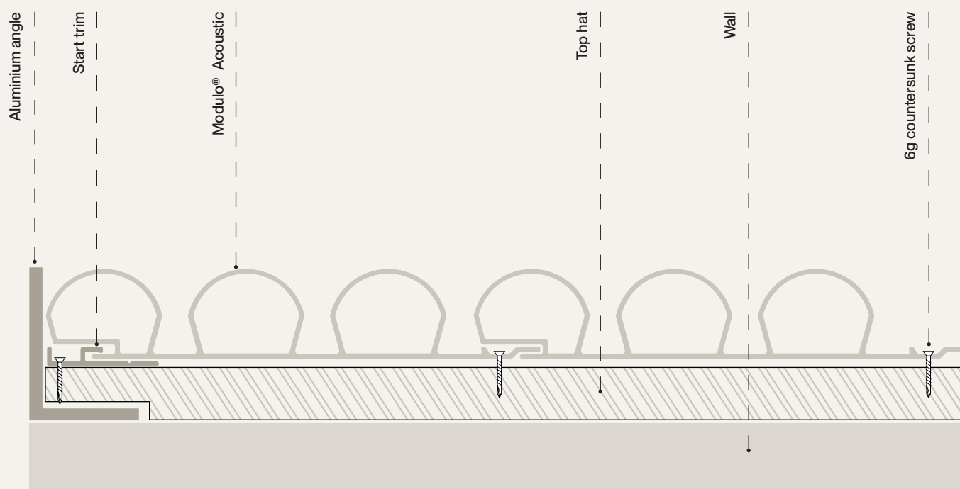
Figure 4. Section view of concealed screw installation of Modulo® Acoustic
