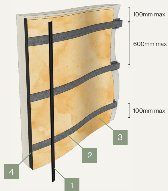
Figure 7. Top hat at 600mm apart, aluminium trim and start trim
