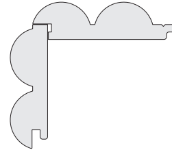
Rebated Corner Detail
