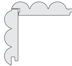
Rebated Corner Detail
