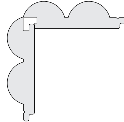
Rebated Corner Detail
