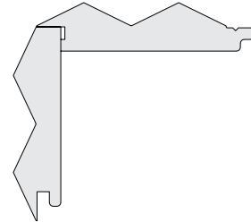
Rebated Corner Detail
