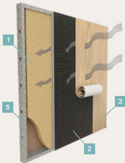
Wall installation
