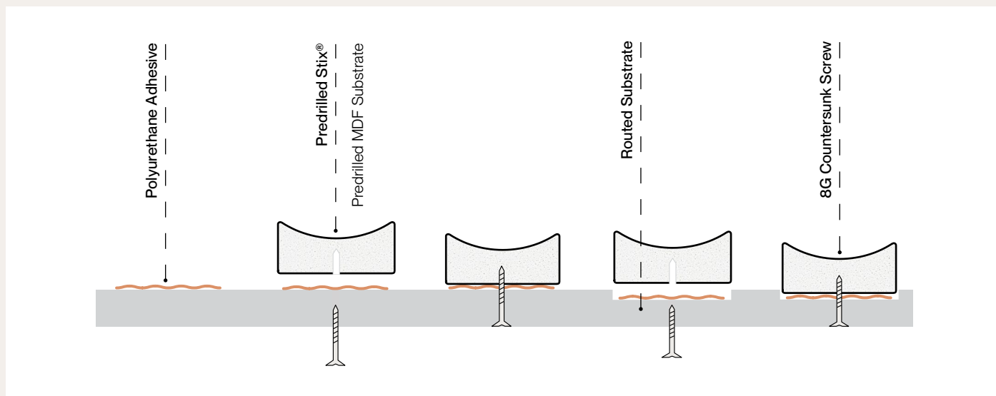
Figure 1. Direct Fix and Rebated Direct Fix, end view
