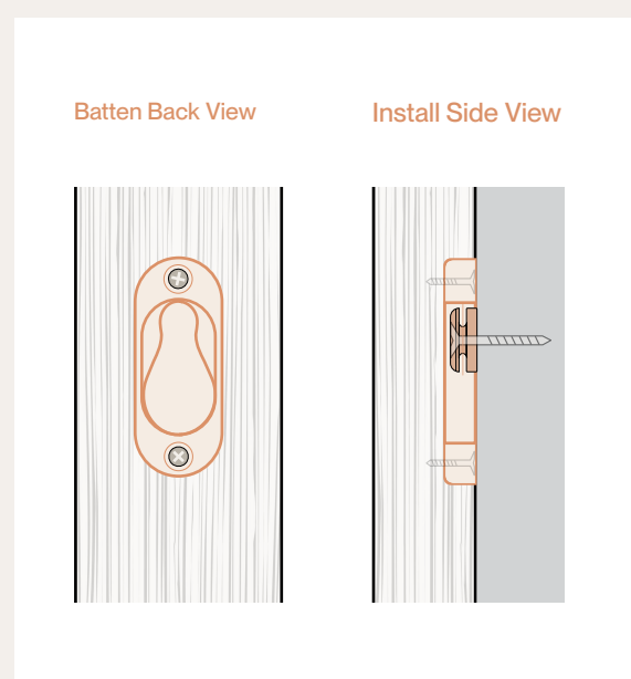
Figure 3. Keyhole/ Button Fix
